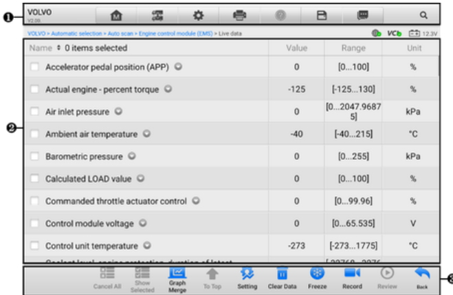
Figure 4-14 Live Data Screen
